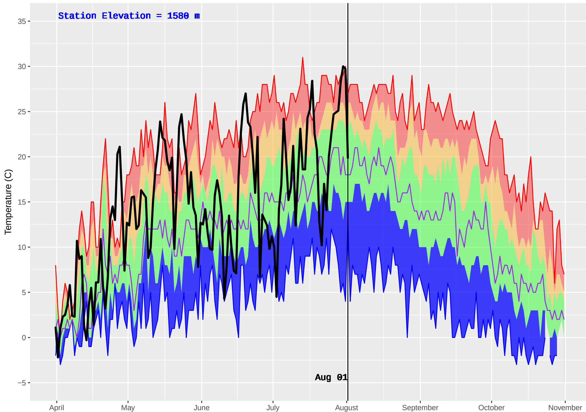
WINDY MOUNTAIN (244) : Historical (1989–2016) and Current (2018) Daily Temperature
