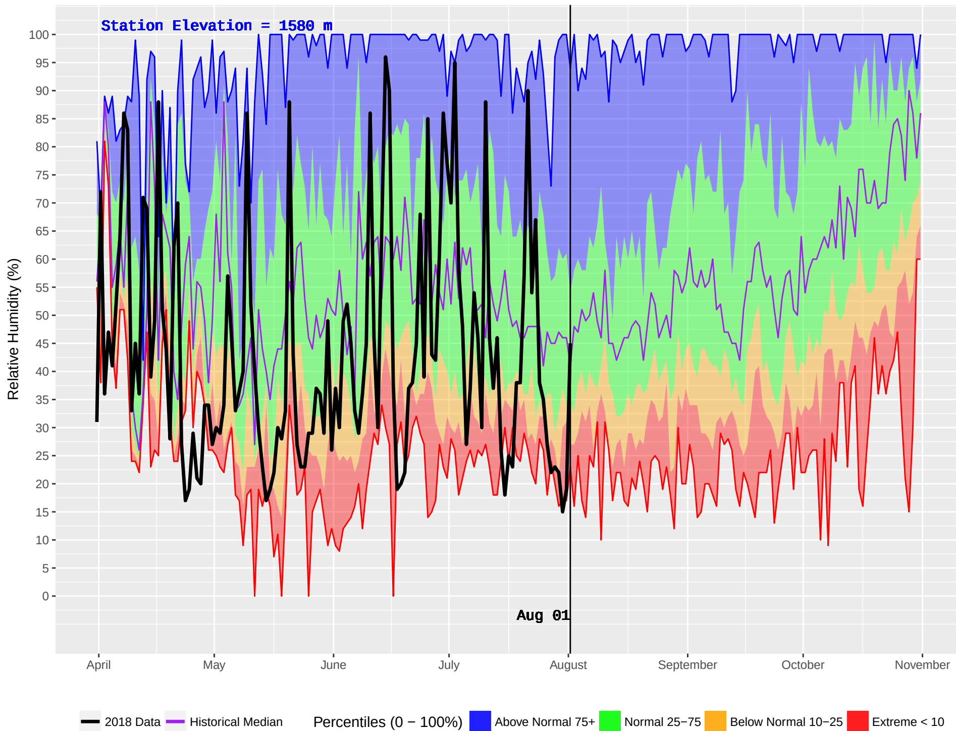
WINDY MOUNTAIN (244) : Historical (1989–2016) and Current (2018) Daily Relative Humidity
